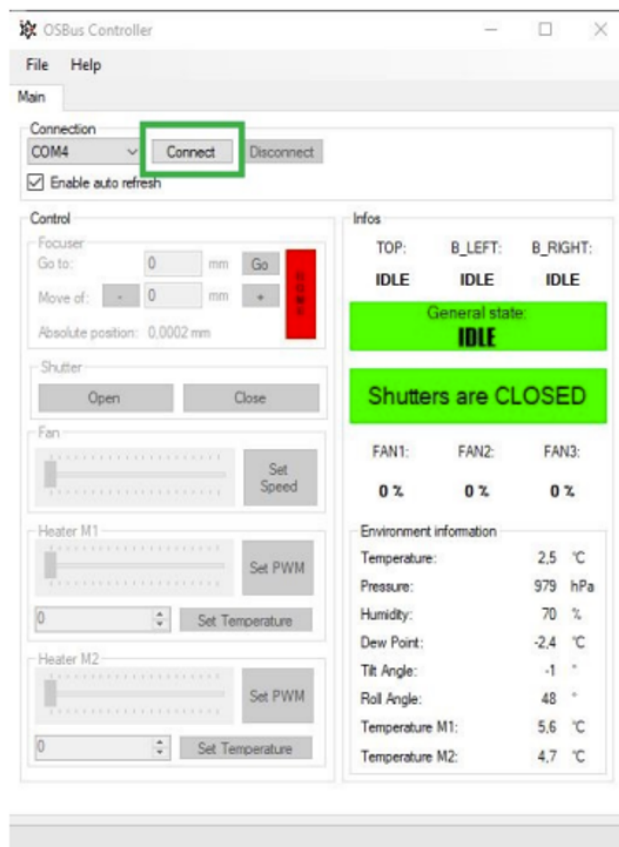
Figure 2.1: OSBus main tab
