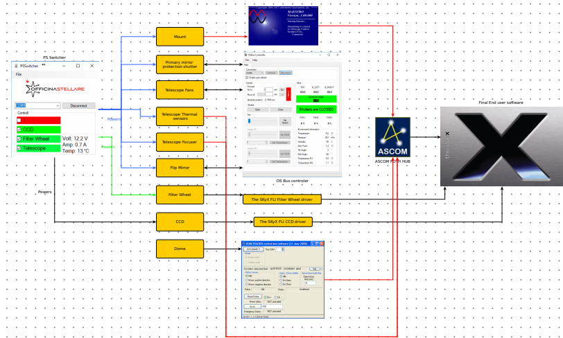
Figure 2.4: TELESTO softwares interactions
