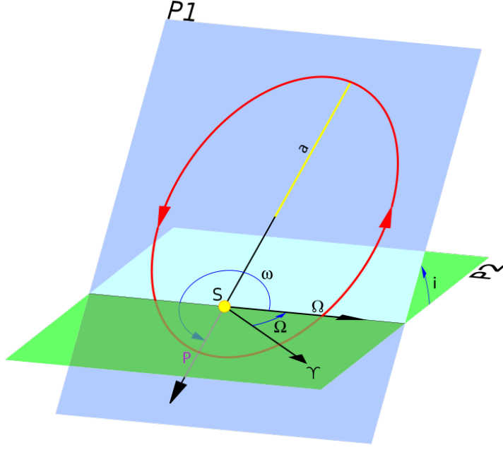
Figure 3.1: Orbital elements: a semi-major axis, e eccentricity, i inclination, \Omega right ascension of ascending node, \omega perigee, \nu true anomaly, E eccentric anomaly, M mean anomaly
